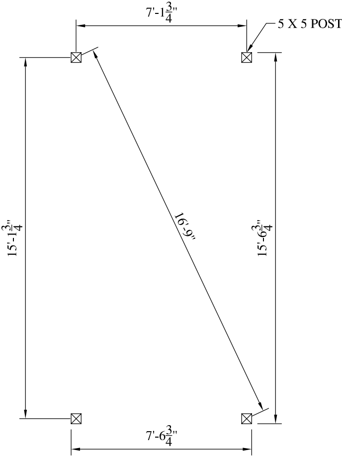
8' X 16' POST LAYOUT PLAN SCALE: 1/4" = 1'-0"
