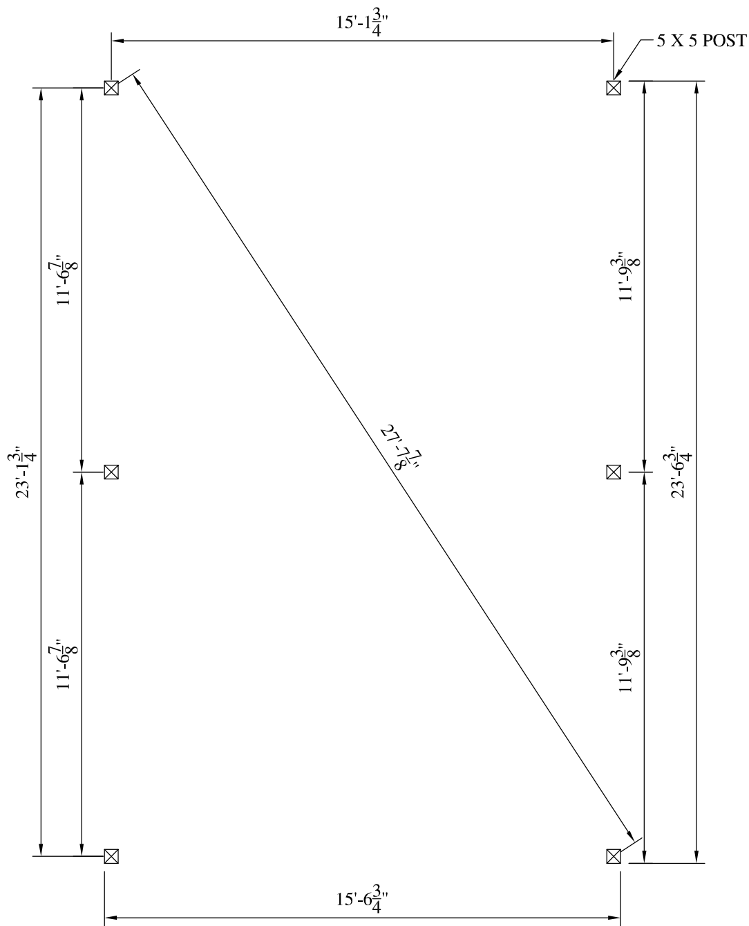
16' X 24' POST LAYOUT PLAN SCALE: 1/4" = 1'-0"
