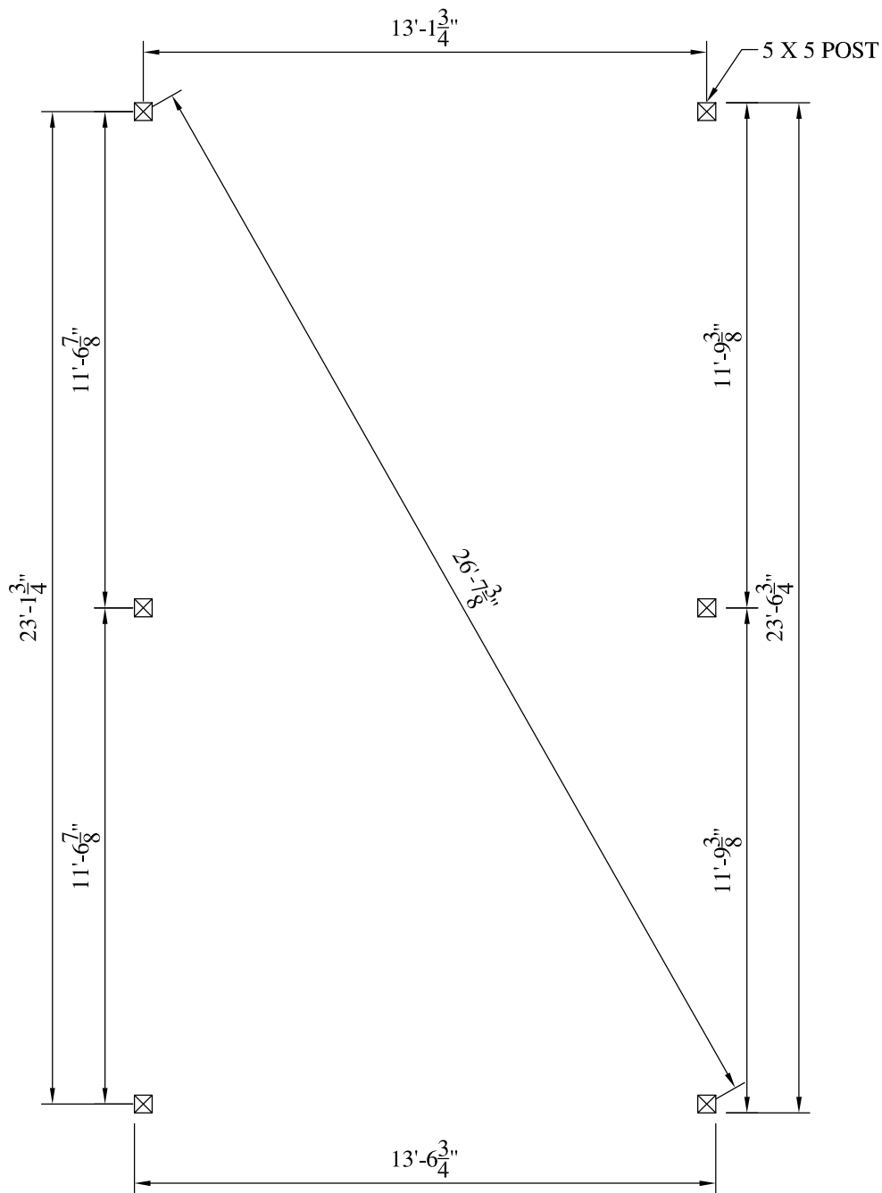
14' X 24' POST LAYOUT PLAN SCALE: 1/4" = 1'-0"
