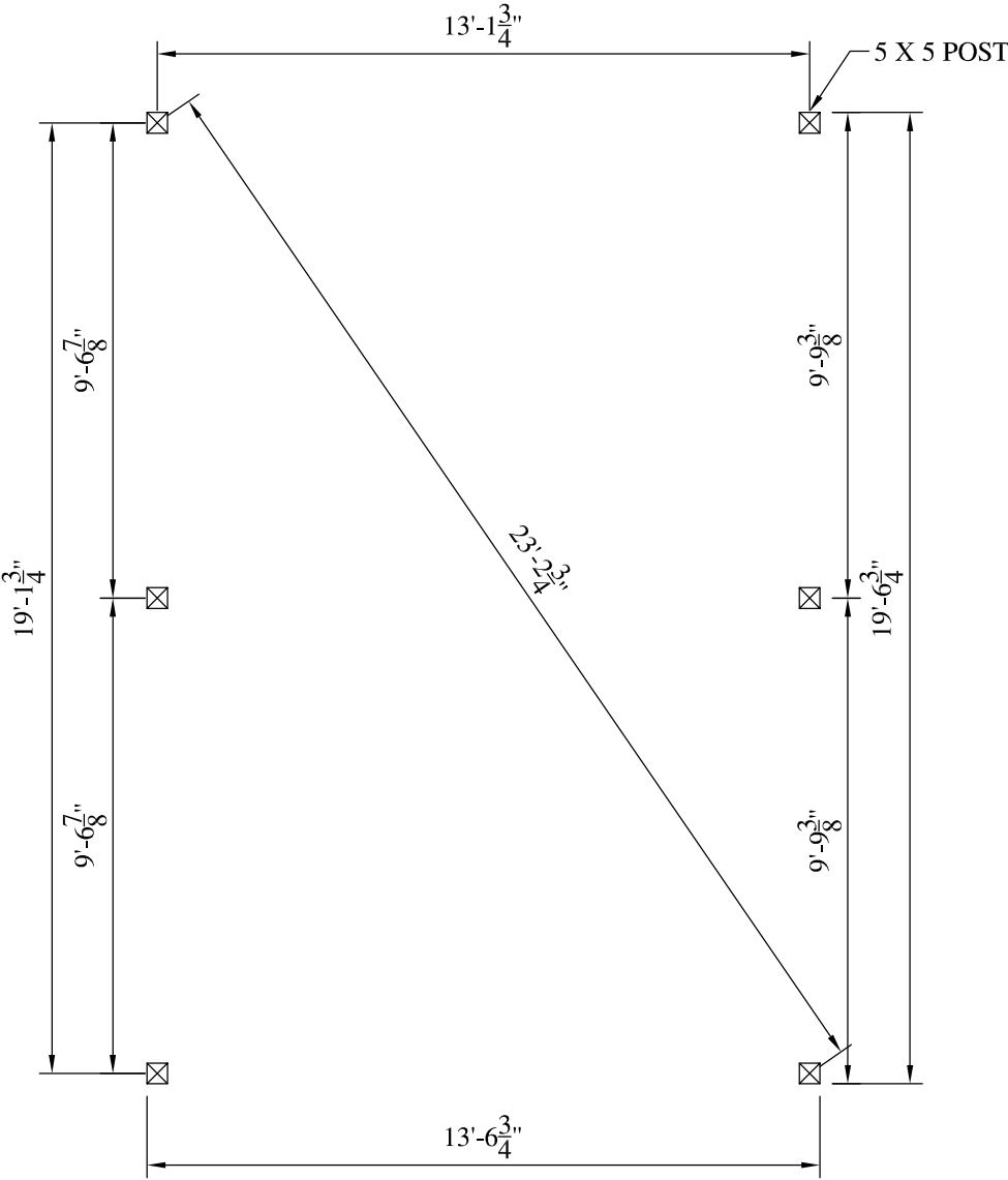
14' X 20' POST LAYOUT PLAN SCALE: 1/4" = 1'-0"
