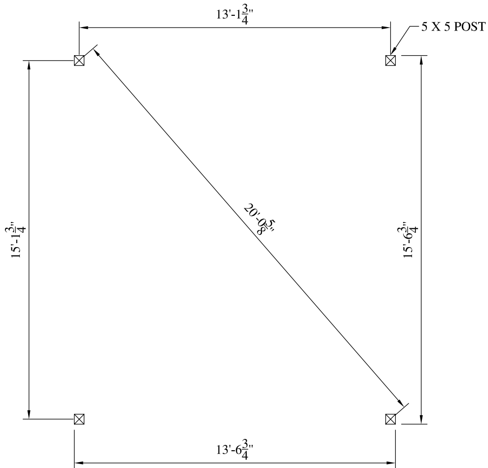
14' X 16' POST LAYOUT PLAN SCALE: 1/4" = 1'-0"
