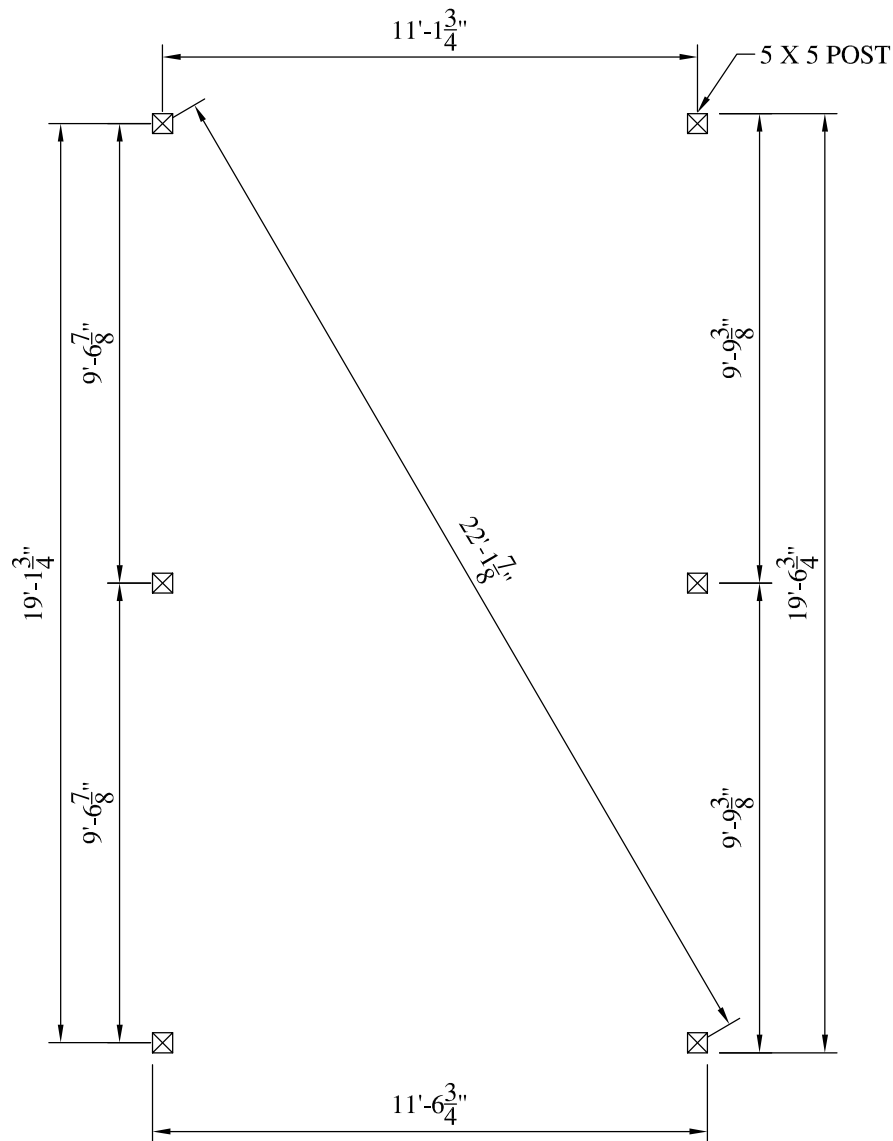
12' X 20' POST LAYOUT PLAN SCALE: 1/4" = 1'-0"
