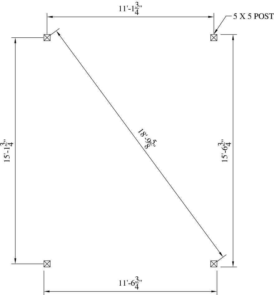
12' X 16' POST LAYOUT PLAN SCALE: 1/4" = 1'-0"
