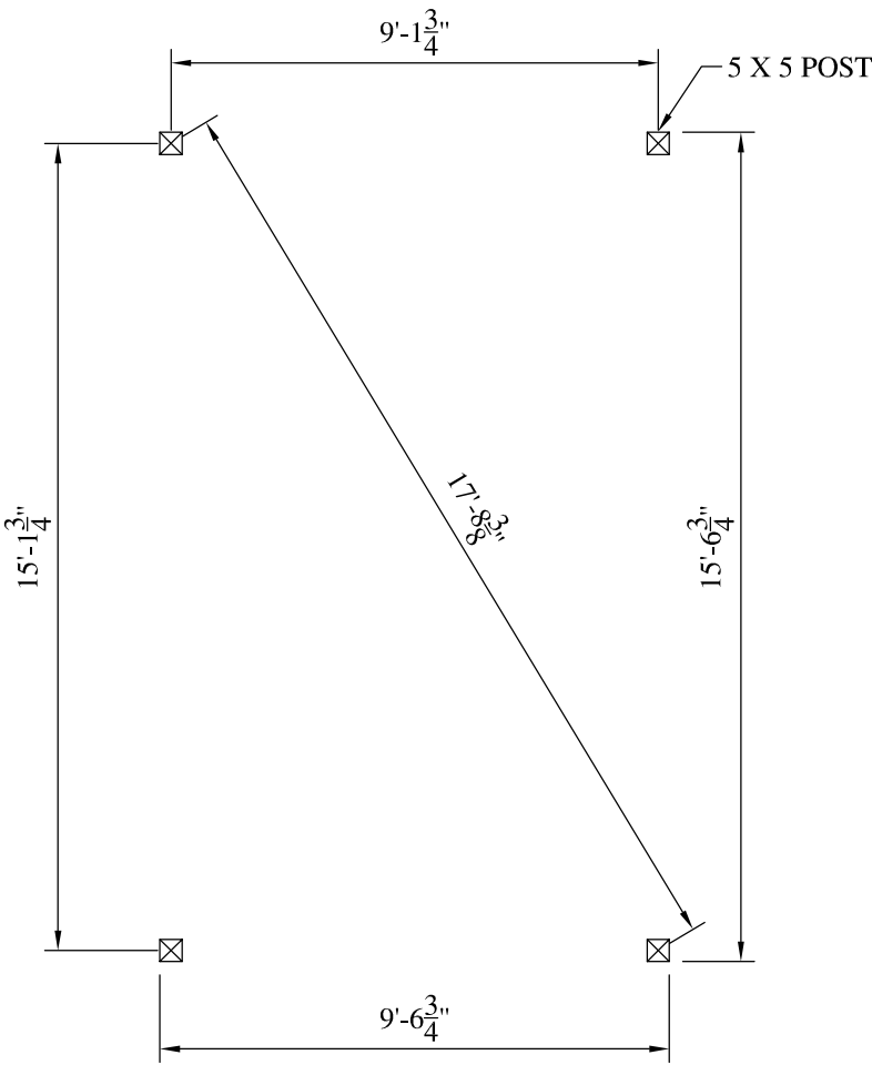
10' X 16' POST LAYOUT PLAN SCALE: 1/4" = 1'-0"
