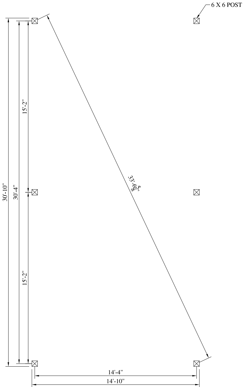
16' X 32' POST LAYOUT PLAN SCALE: 1/4" = 1'-0"
