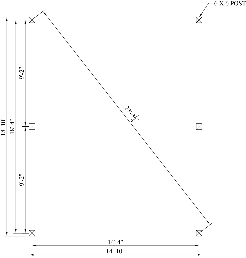
16' X 20' POST LAYOUT PLAN SCALE: 1/4" = 1'-0"
