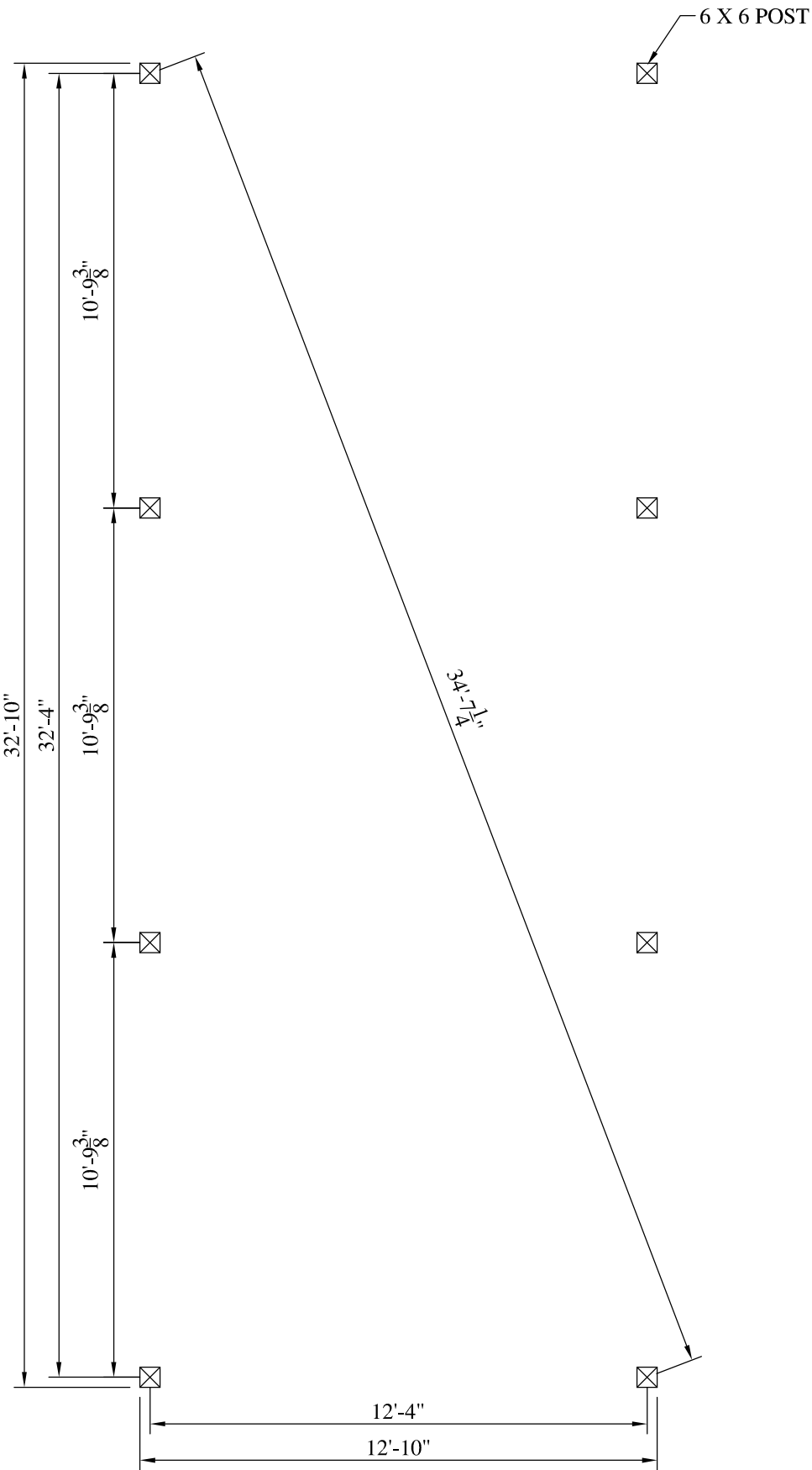
14' X 34' POST LAYOUT PLAN SCALE: 1/4" = 1'-0"
