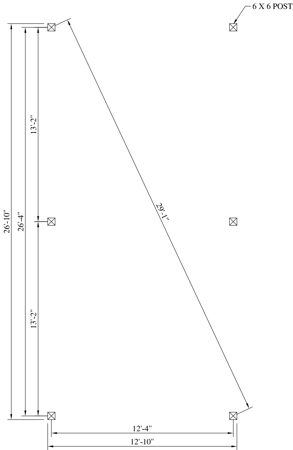
14' X 28' POST LAYOUT PLAN SCALE: 1/4" = 1'-0"
