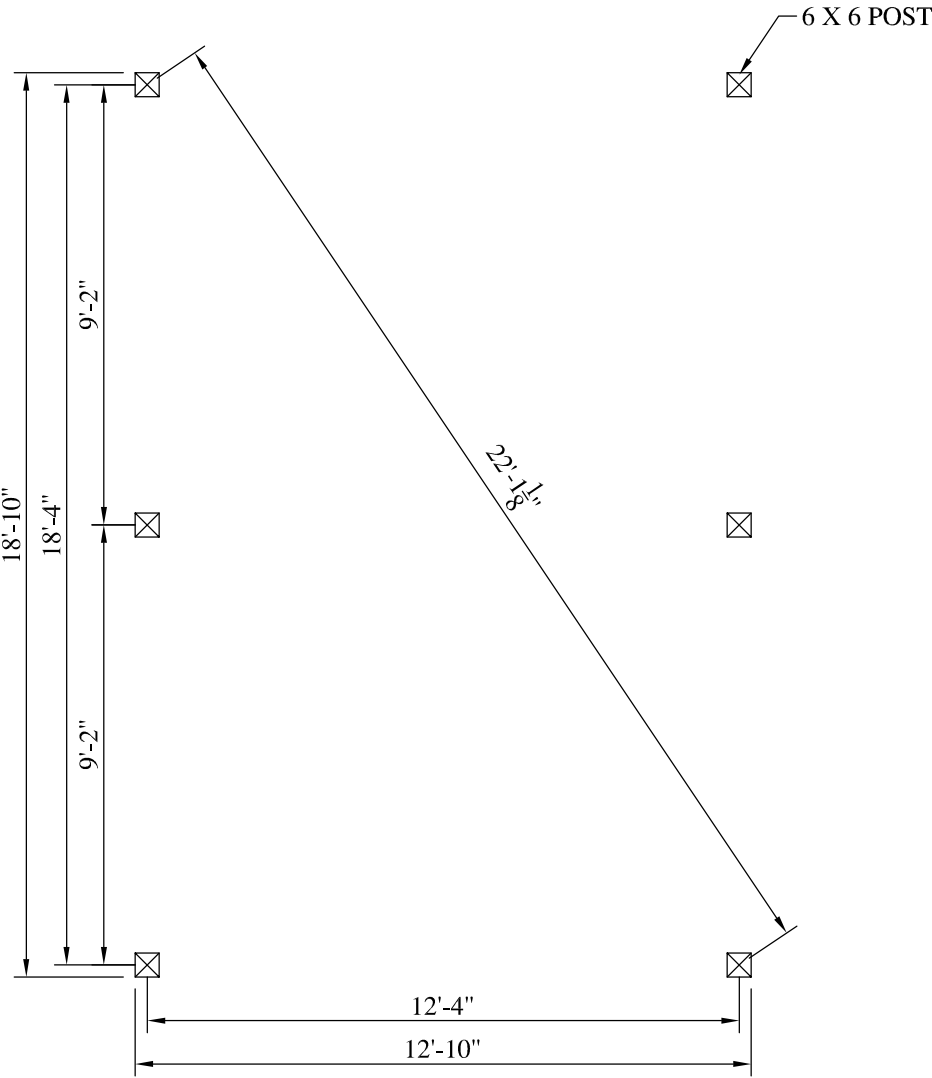
14' X 20' POST LAYOUT PLAN
