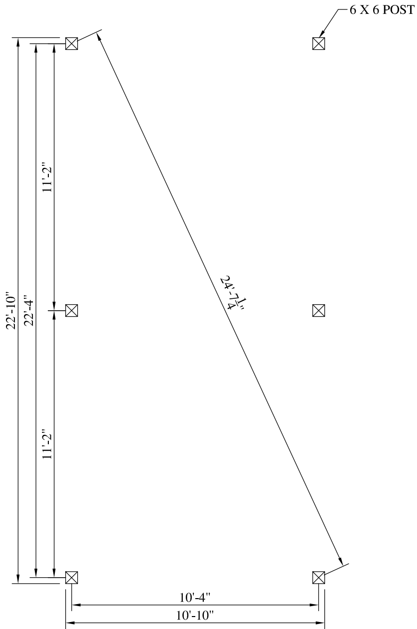
12' X 24' POST LAYOUT PLAN SCALE: 1/4" = 1'-0"
