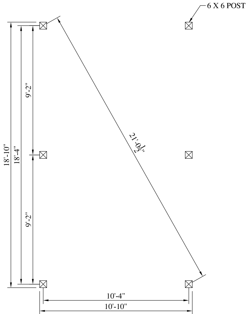
12' X 20' POST LAYOUT PLAN SCALE: 1/4" = 1'-0"
