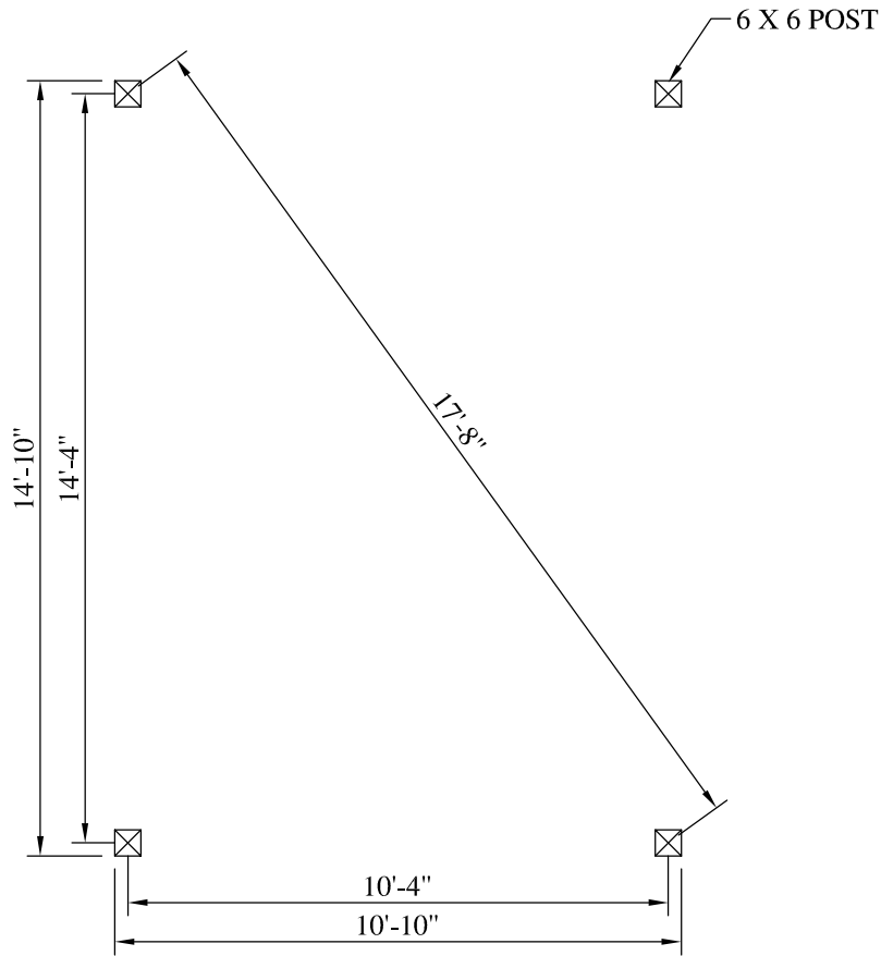
12' X 16' POST LAYOUT PLAN SCALE: 1/4" = 1'-0"
