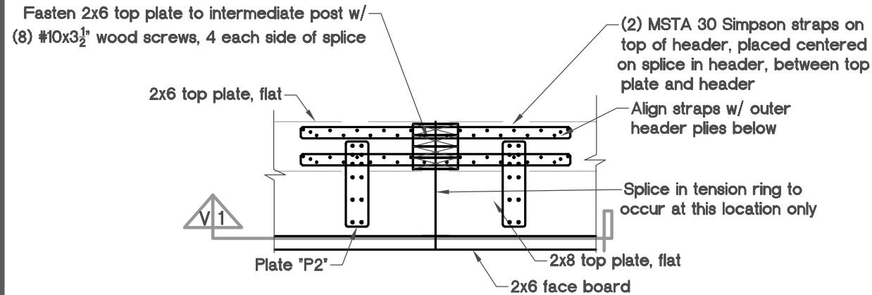
Detail G-G/10
