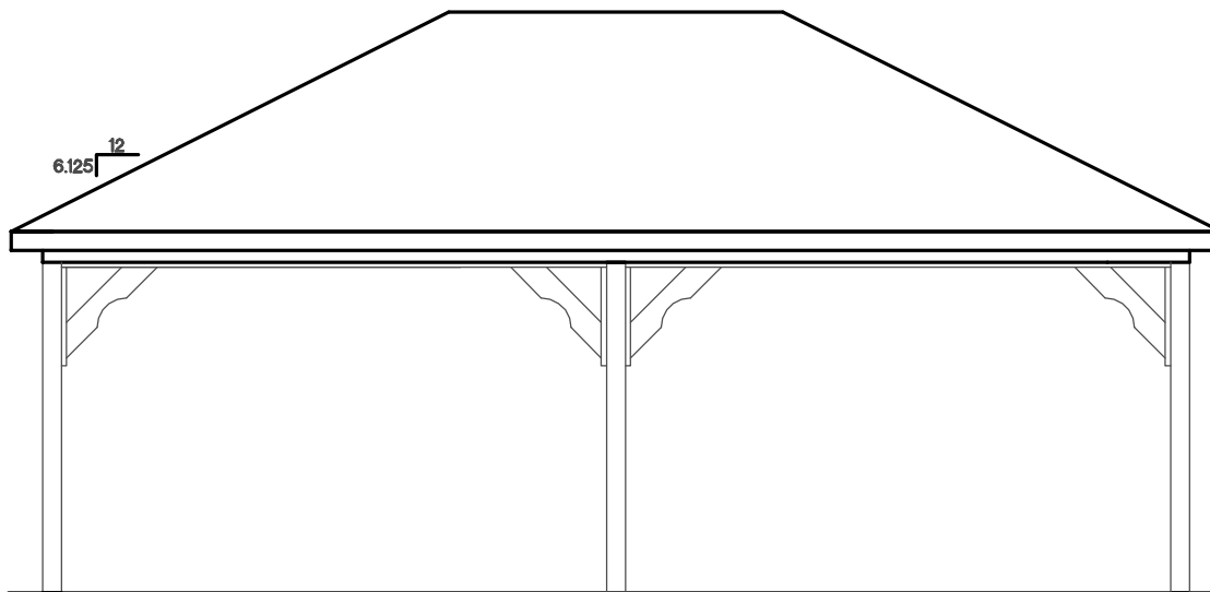
Side Elevation
