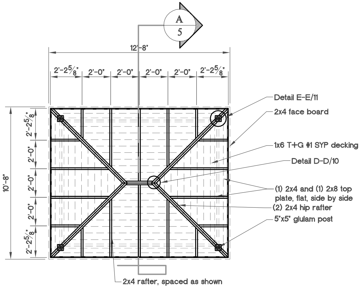
Roof Framing Plan Scale 1/4" = 1'-0"
