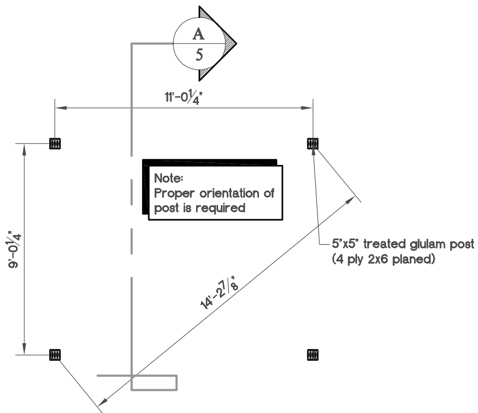
Post Layout Plan Scale \frac{1}{4}" = 1'-0"
