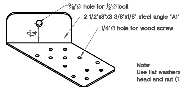
Angle "A1"
