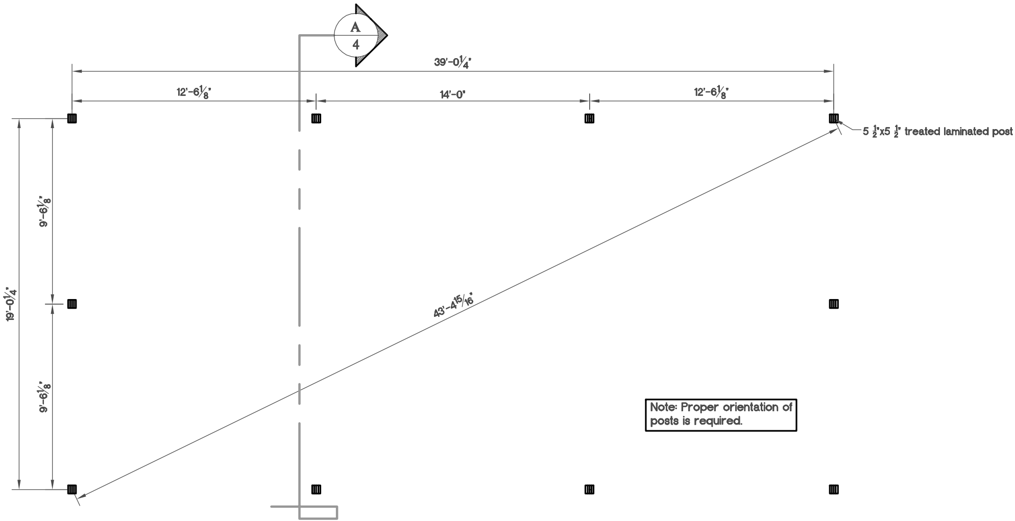
Post Layout Plan
