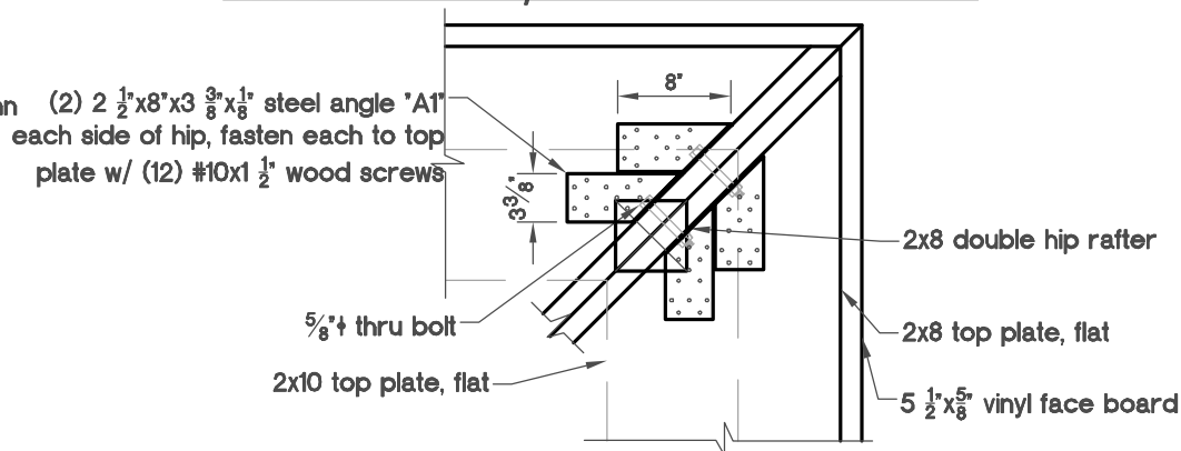
Detail E-E/7
