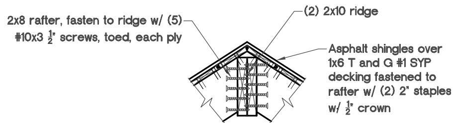
Detail A-A/4 Typical Single Rafter NTS
