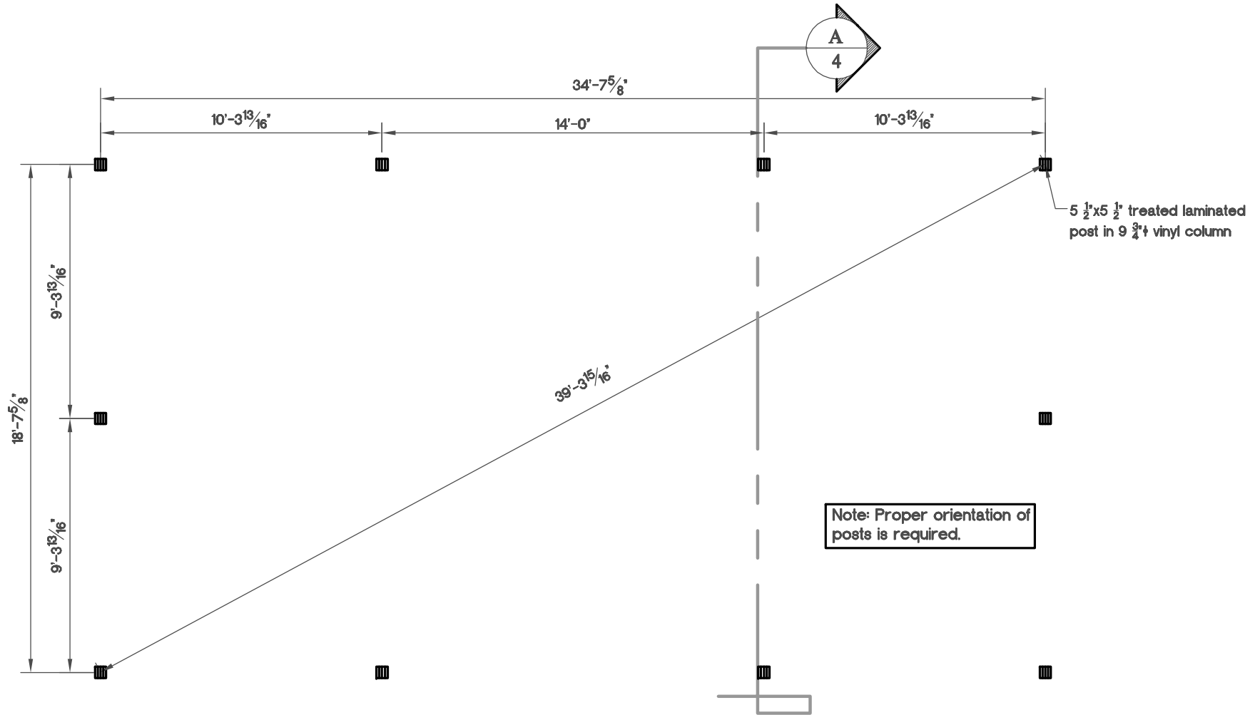
Post Layout Plan
