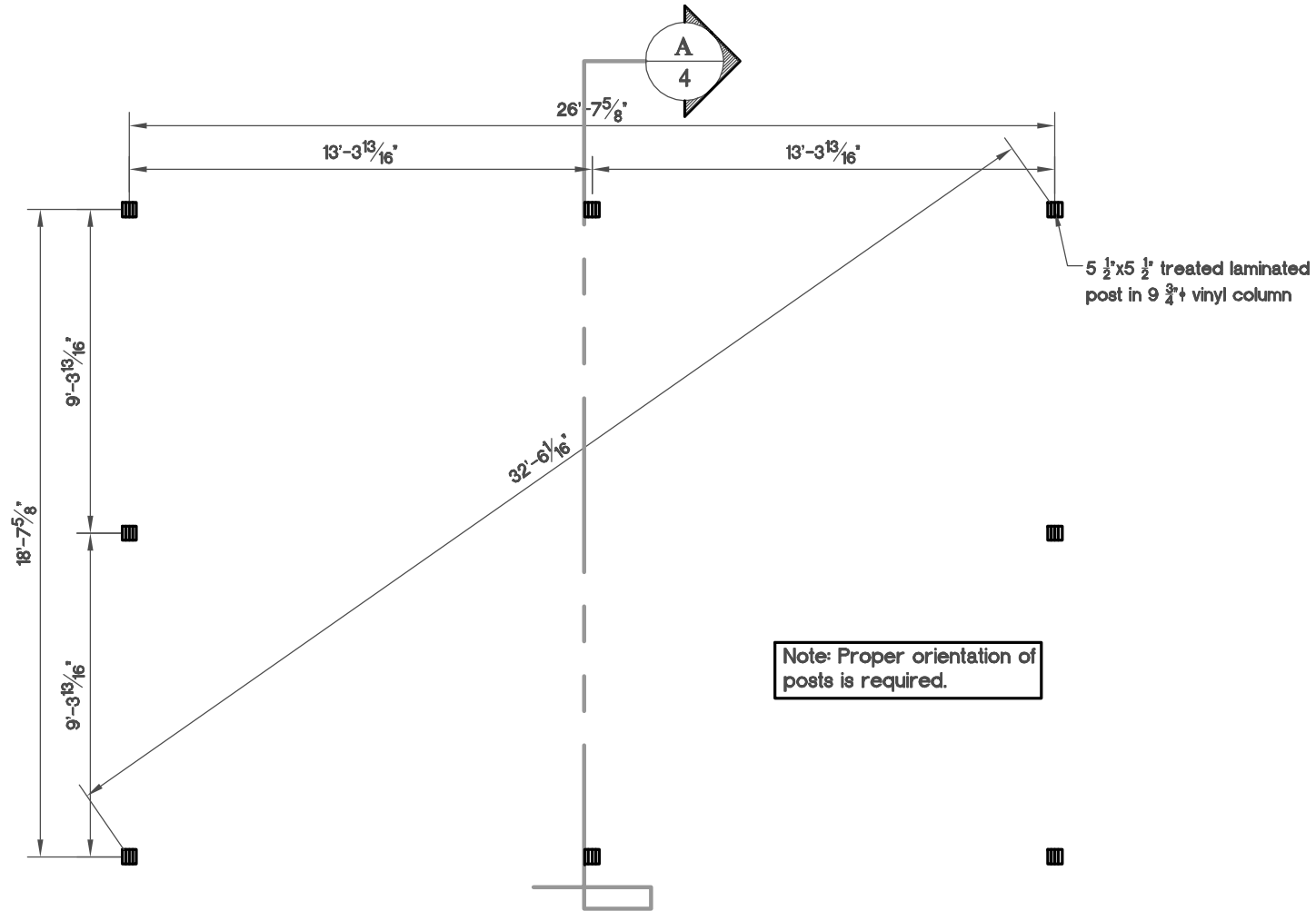
Post Layout Plan
