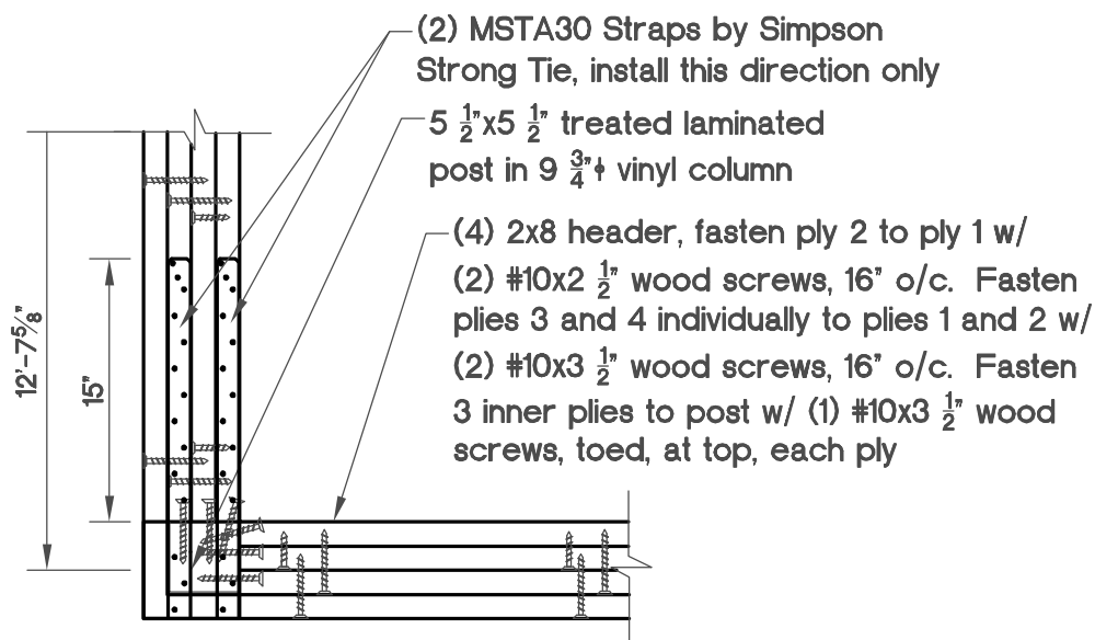
View 2 Detail B-B/6
